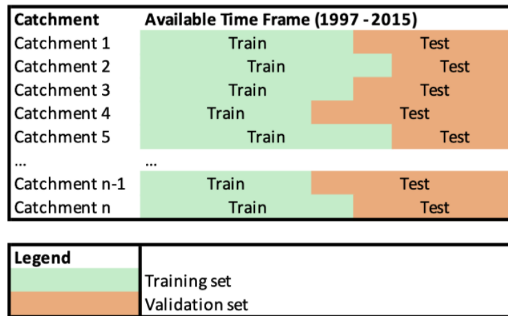
Fig. 2: Train-test split
